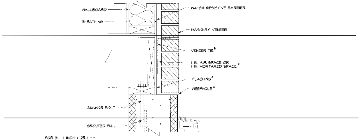
FIGURE R 703.8 MASONRY VENEER WALL DETAILS (CONTINUED)
