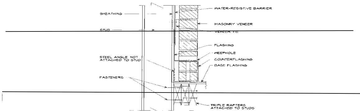
SUPPORT BY ROOF CONSTRUCTION FIGURE R 703.8.2.2 EXTERIOR MASONRY VENEER SUPPORT BY ROOF CONSTRUCTION
