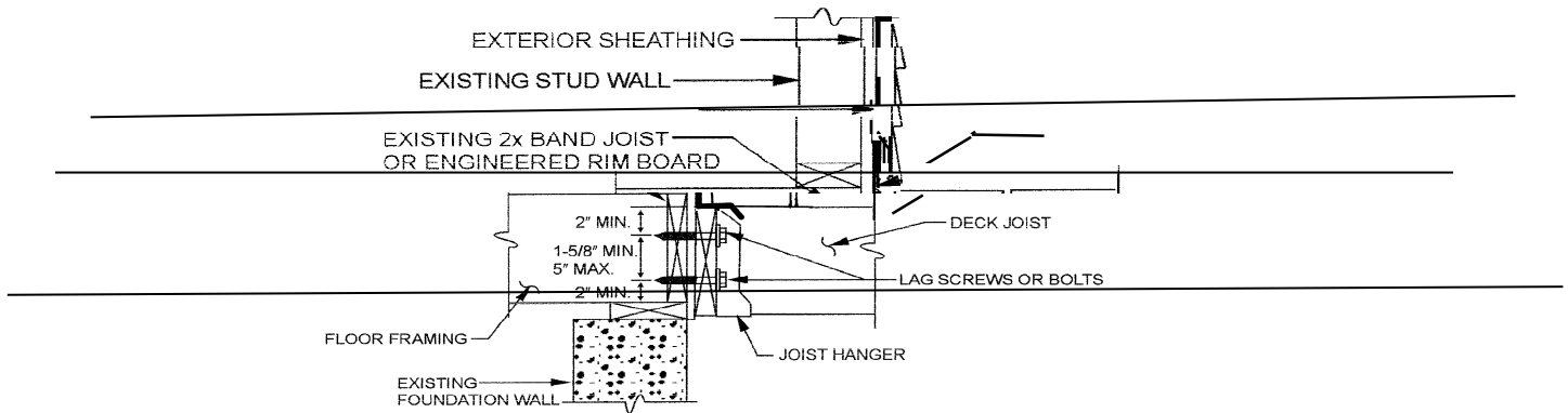
FIGURE R507.2.1(2) PLACEMENT OF LAG SCREWS AND BOLTS IN BAND JOISTS
